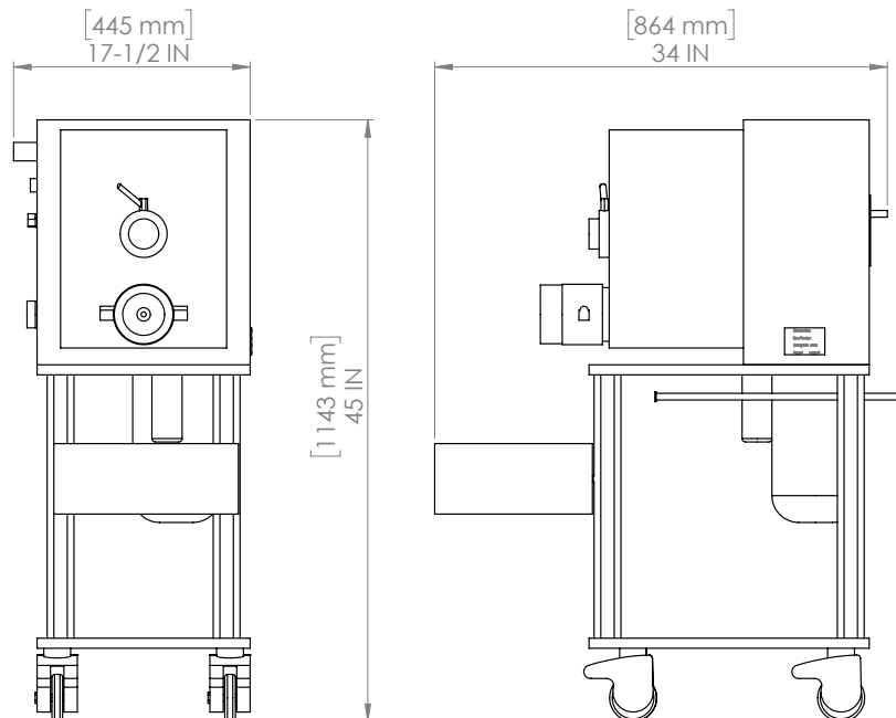
AMFE 50 Extruder & Mixer
