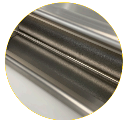
KNURLED ROLLERS FOR TEXTURE LIKE RUSTIC EXTRUDED PASTA 0 - 5/8" OPENING
